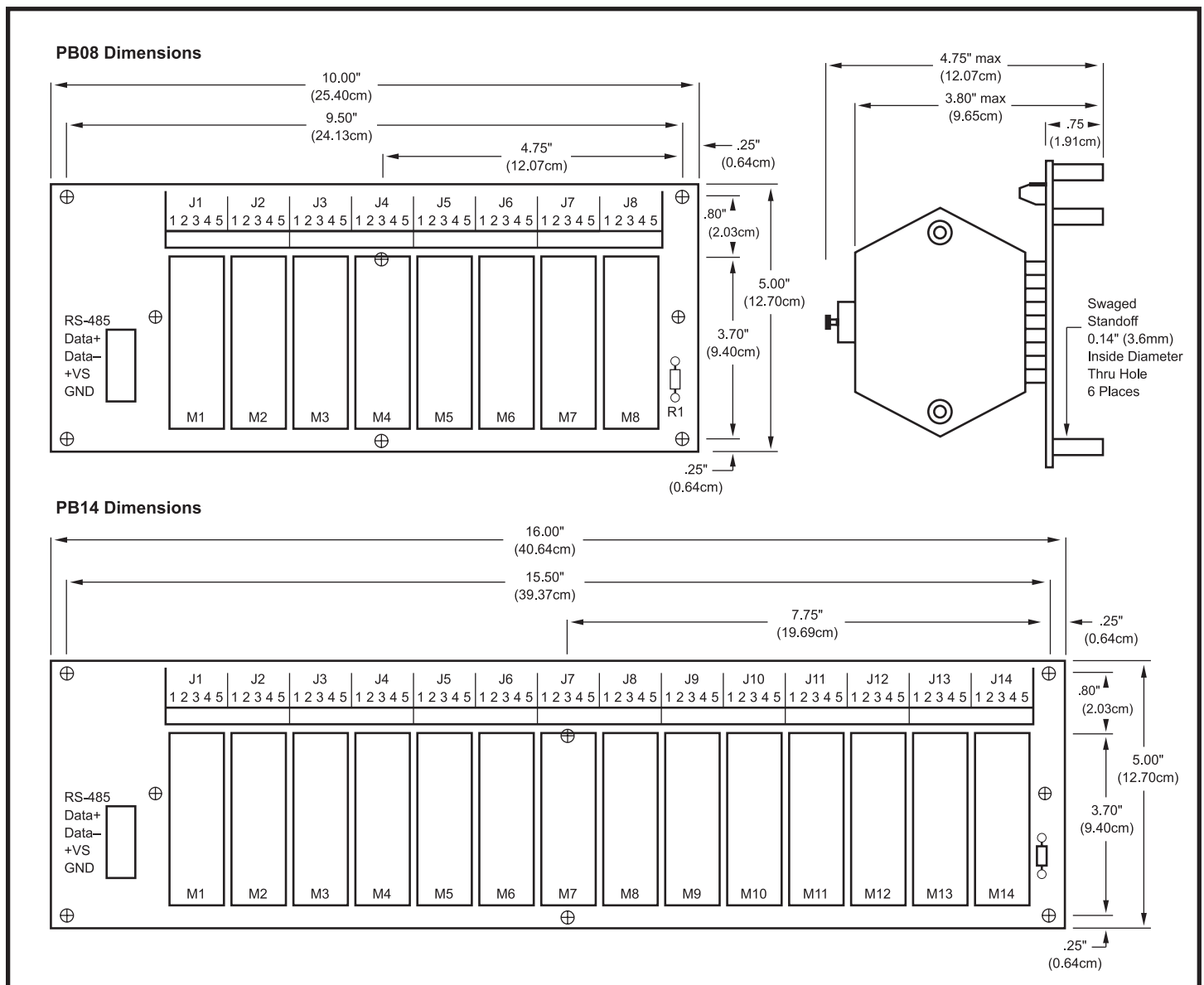
Figure 1: SCM9B-PB08/PB14 Dimensions
