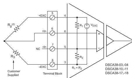
Figure 3: Quarter Bridge Connection
