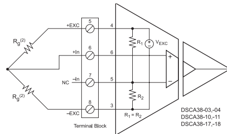
Figure 2: Half Bridge Connection
